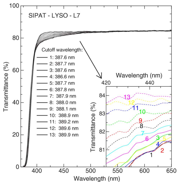
Fig. 4. Transverse transmittance spectra measured every 2 cm from the seed (curve-1) to the tail (curve-13) end are shown as a function of wavelength for SIPAT-LYSO-L7. The inset is an expanded view between 420 nm and 450 nm.
