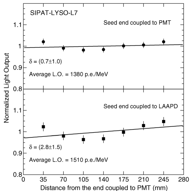
Fig. 6. Normalized light output (black dots) is shown as a function of distance to the photo-detector for SIPAT-LYSO-L7. Also shown are the linear fit and corresponding average light output and light response uniformity ( \delta ) as defined in equation (3).
