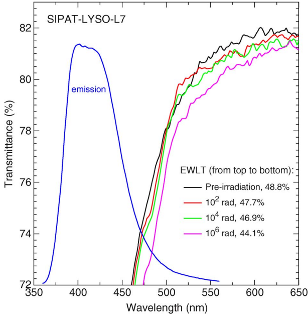
Fig. 7. Expanded view of the longitudinal transmittance spectra measured before and after \gamma -ray irradiations in several steps up to 1 Mrad is shown for SIPAT-LYSO-L7. Also shown is the emission spectrum and the values of EWL defined in the text.
