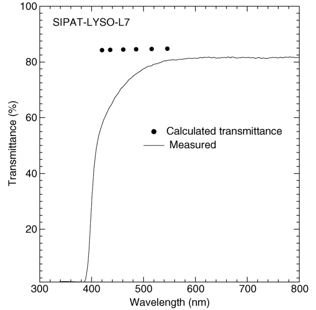
Fig. 3. Longitudinal transmittance spectrum (black lines) is shown as a function of wavelength for SIPAT-LYSO-L7 together with the theoretical limits (black dots).
