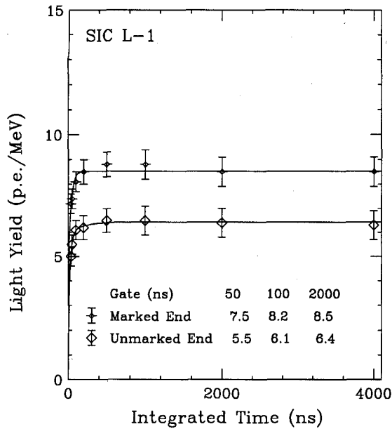
Fig. 6 Light output of sample SIC L-1 is plotted as a function of integration time, showing different amplitudes when different ends of the sample were coupled to the PMT.
