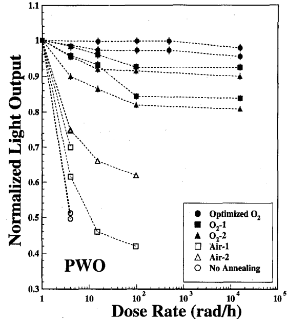
Fig. 2 Normalized light output degradation is shown as a function of the dose rate for samples prepared under different annealing conditions.
