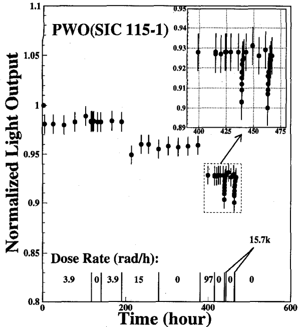
Fig. 1 The normalized light output of sample 115-1 is shown as a function of time and dose rate.
