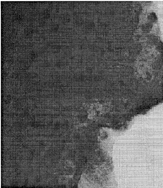
Fig. 8 TEM picture of a \text{PbWO}_4 sample with poor radiation hardness, showing black spots of \phi 5\text{--}10 nm related to oxygen vacancies.
