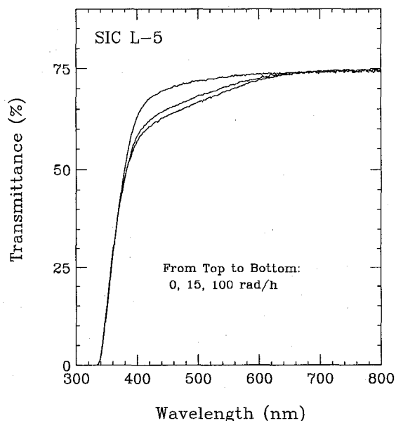
Fig. 5 Transmittance at equilibrium at different dose rates is shown as a function of wavelength for sample SIC L-5.
