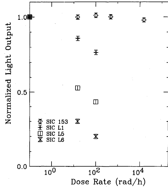
Fig. 7 Normalized light output at equilibrium is shown as a function of dose rate for three La doped samples, and compared to oxygen annealed sample SIC 153.
