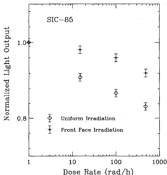
Fig. 4 Light output degradation at equilibrium is shown as a function of dose rate for uniform and front irradiations for sample SIC 85.
