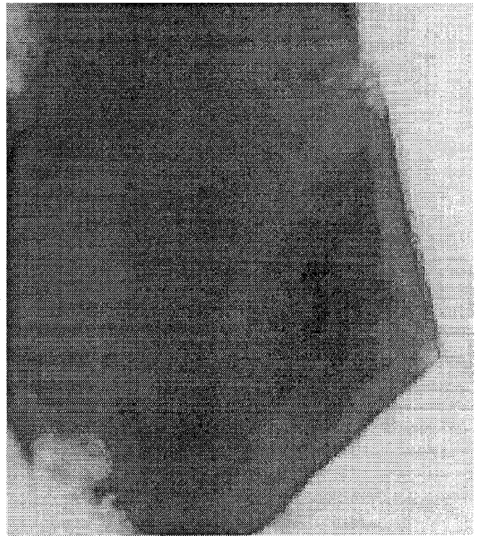
Fig. 9 TEM picture of a \text{PbWO}_4 crystal with good radiation hardness, showing no black spots.
