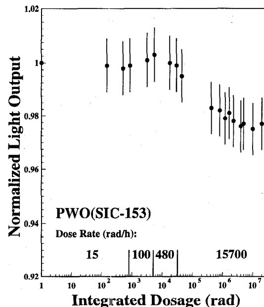
Fig. 3 The normalized light output of sample SIC 153 is shown as a function of integrated dose.
