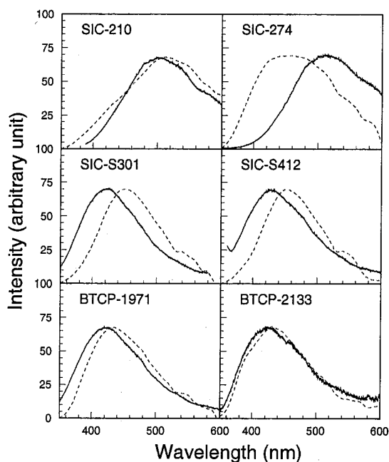
Figure 3: A comparison of photo (solid) and radio (dashed) luminescence spectra for six PbWO 4 samples.
