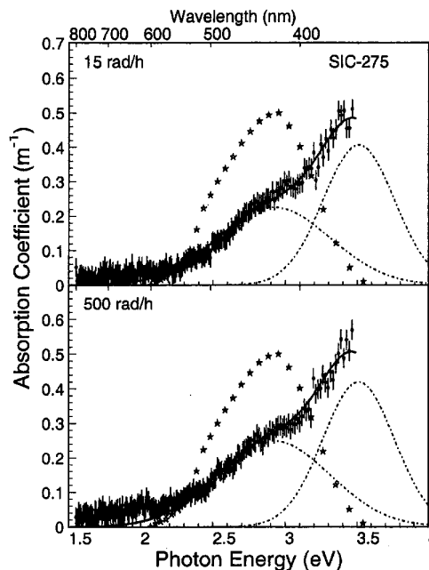
Figure 5: Radiation induced color center density for a Sb doped sample SIC-275.
