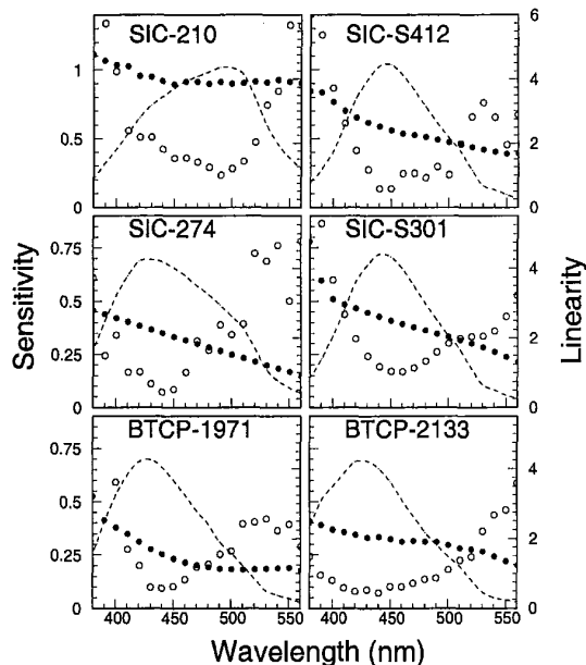
Figure 14: Monitoring sensitivity and linearity are shown as function of wavelength for six \text{PbWO}_4 samples.
