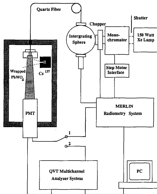
Figure 11: The monitoring test bench for light monitoring (position 1) and light output measurement (position 2).
