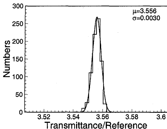
Figure 12: Distribution of PMT readout (position 1) normalized to reference detector on sphere, taken in 23 hours is shown with a Gaussian fit.
