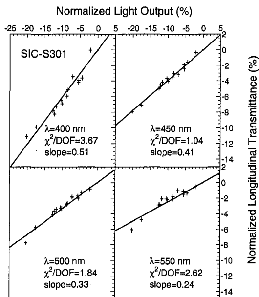
Figure 13: Correlations between relative variations of transmittance and light output are shown for four monitoring wavelengths for a Y/Sb double doped sample SIC-S301.
