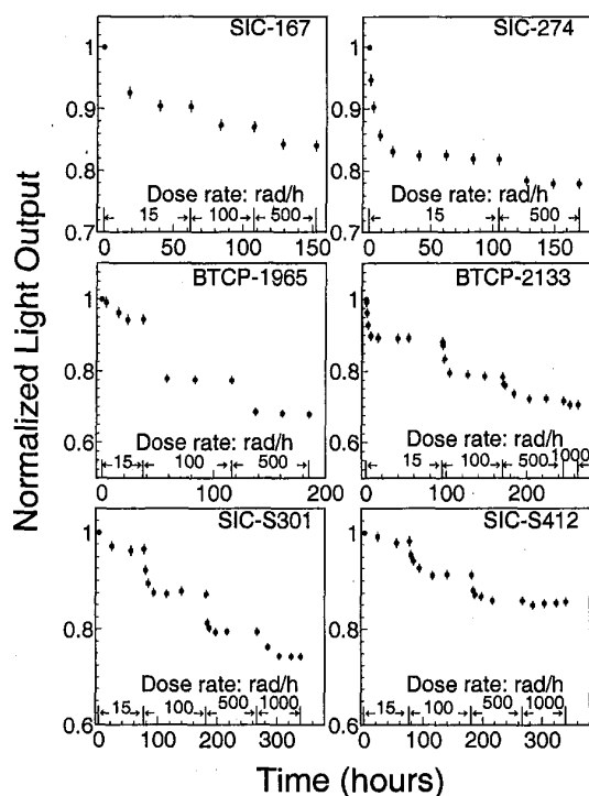
Figure 10: Normalized light output is shown as function of time after irradiation for six PbWO_4 crystals.
