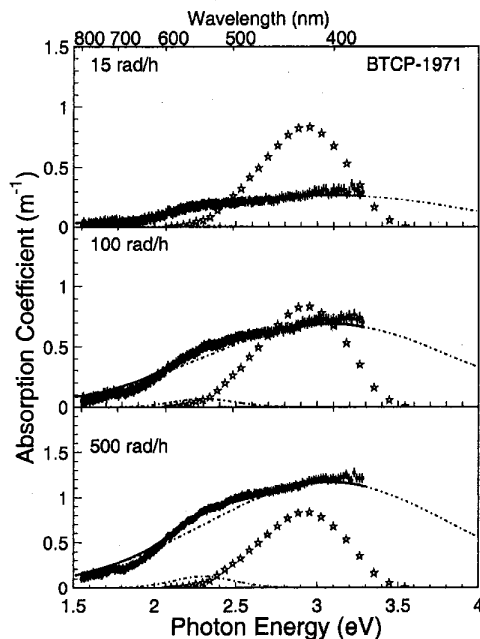
Figure 6: Radiation induced color center density for a La doped sample BTCP-1971.
