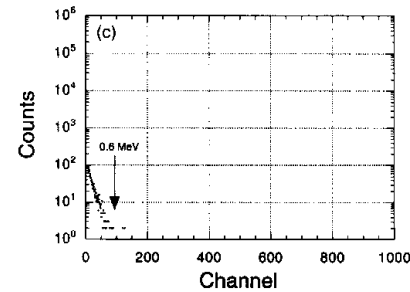
Fig. 3. Pulse height distribution for ^{252}\text{Cf} neutrons. (a) with a polyethylene radiator (thickness = 45 \mu\text{m} ). (b) without polyethylene radiator. (c) background in case of no neutron source.
