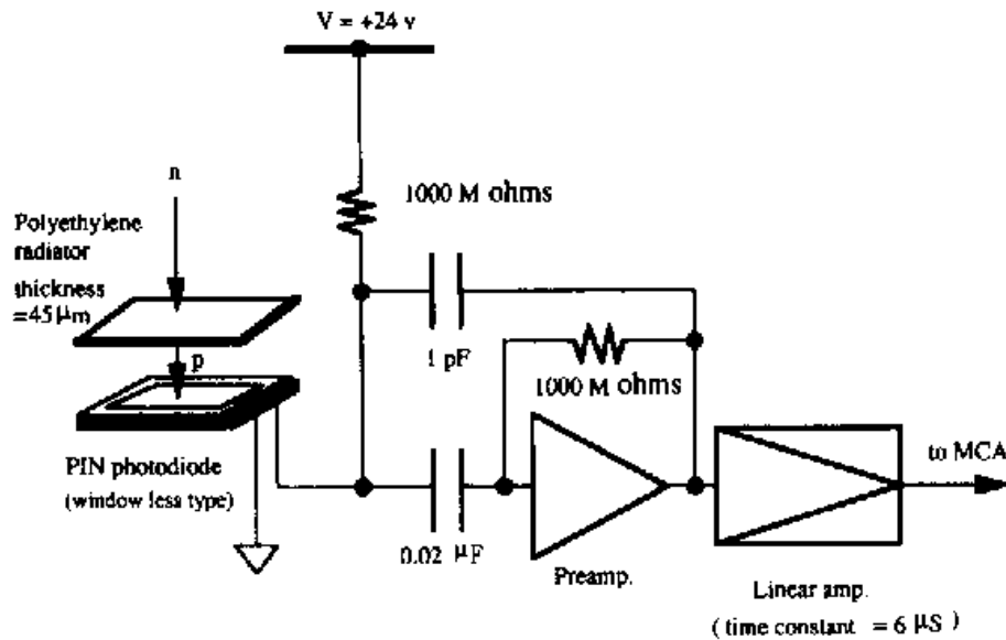
Fig. 1. Block diagram of the fast neutron PD detector.
